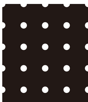
65 3.0φ × 10.0P 開孔率 7.1%
