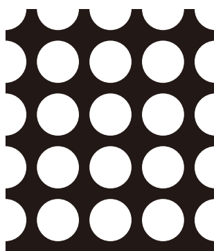
74 8.0φ × 10.0P 開孔率 50.2%
